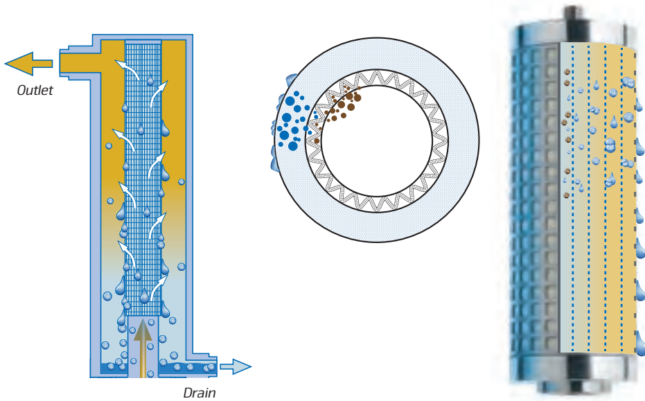
Inner setup coalescer element
