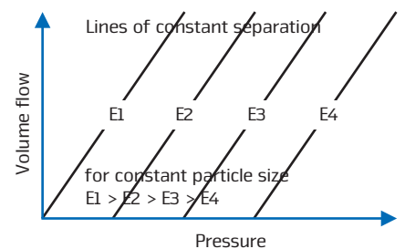
ISO - separation efficiency curve - principle
